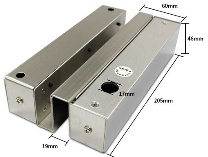
205mm length version (if your bolt lock's length is 205mm, then take this size)
