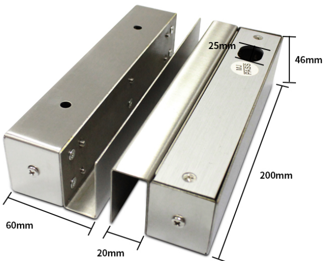
200mm length version (if your bolt lock's length is 200mm, then take this one)
